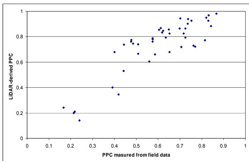
Figure 4: Scatter plot of the PPC estimations from the LiDAR data vs the PPC measurements extracted from upward looking photos.
