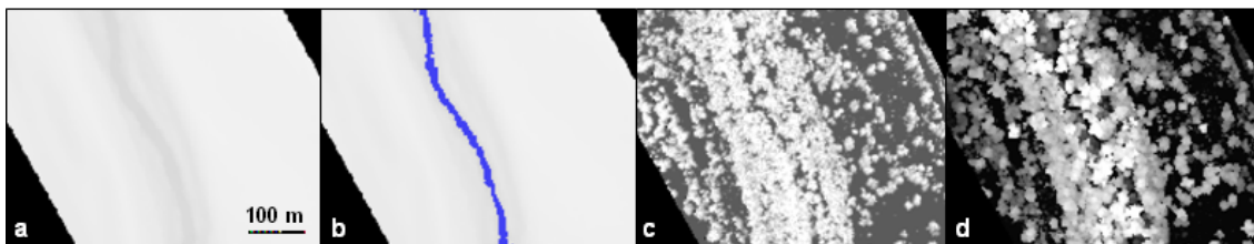
Figure 3: LiDAR-derived products: (a) DTM; (b) streambed map (in blue); (c) PPC and (d) TCM. Bright areas correspond to high values for the terrain elevation (a, b), PPC (c) and tree heights (d).
